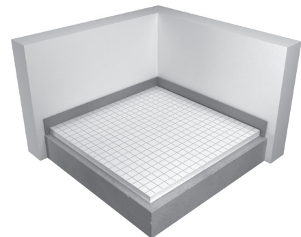
Install the perimeter strip and the Clypso insulation
