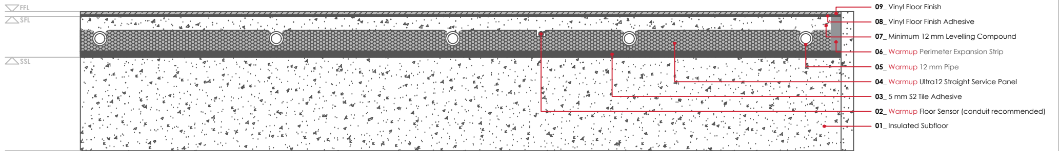
WARMUP ULTRA12 SYSTEM. Vinyl floor finish - glued
