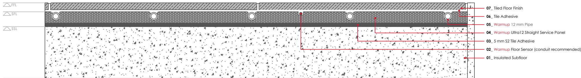
WARMUP ULTRA12 SYSTEM. Tiled floor finish
