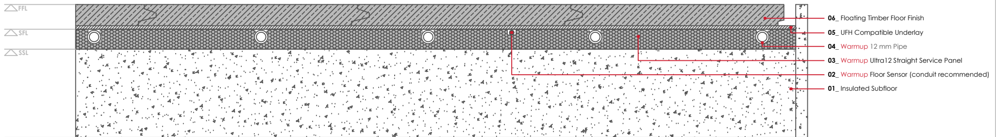
WARMUP ULTRA12 Floating timber floor finish
