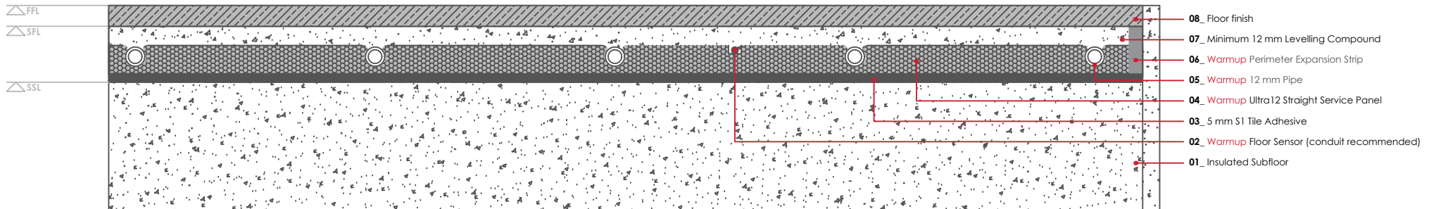
WARMUP ULTRA12 SYSTEM. Standard Detail
