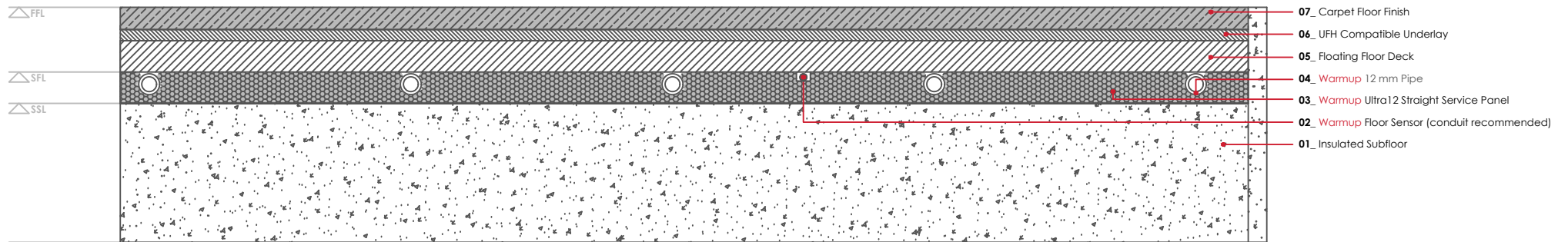
WARMUP ULTRA12 SYSTEM. Carpet floor finish
